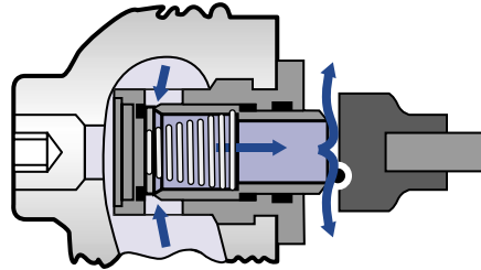
B. Standard Regulator orifice failed; upstream monitor orifice control
