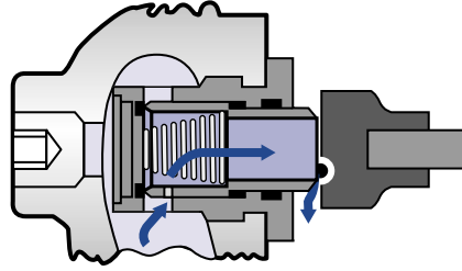
D. "V" Option - Vents small volume of gas to atmosphere through relief valve
